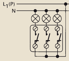
Schalter, 3-polig
